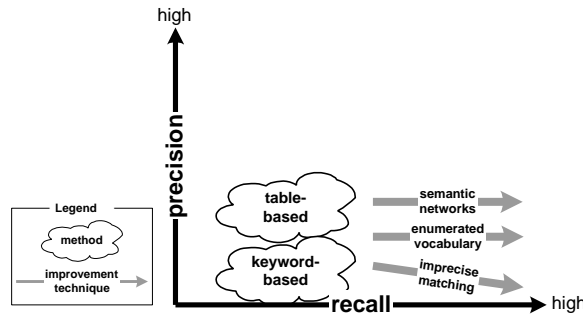
Fig. 1. State of the art in service retrieval
