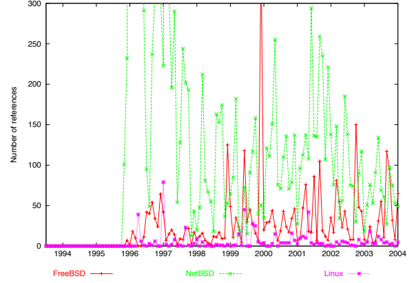
Figure 4: Number of references to keywords FreeBSD , NetBSD , and Linux found in OpenBSD change logs
