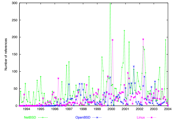
Figure 2: Number of references to keywords NetBSD , OpenBSD , and Linux found in FreeBSD change logs
