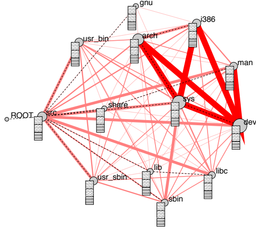
Figure 5: Change coupling between modules of the source code structure of the OpenBSD system
