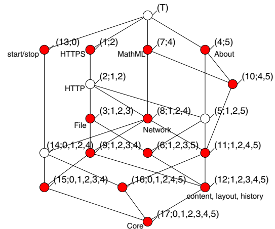
Figure 4. Concept lattice from profile data
