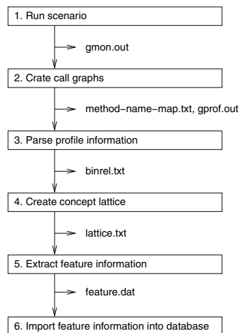
Figure 2. Profiling process
